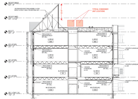
1 A3.01 BUILDING SECTION @ 4 STORY (WEST) 1/8" = 1'-0"
